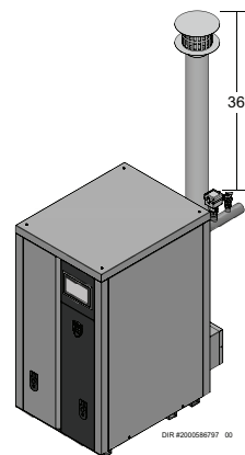
Figure 6-1 Installation extérieure
